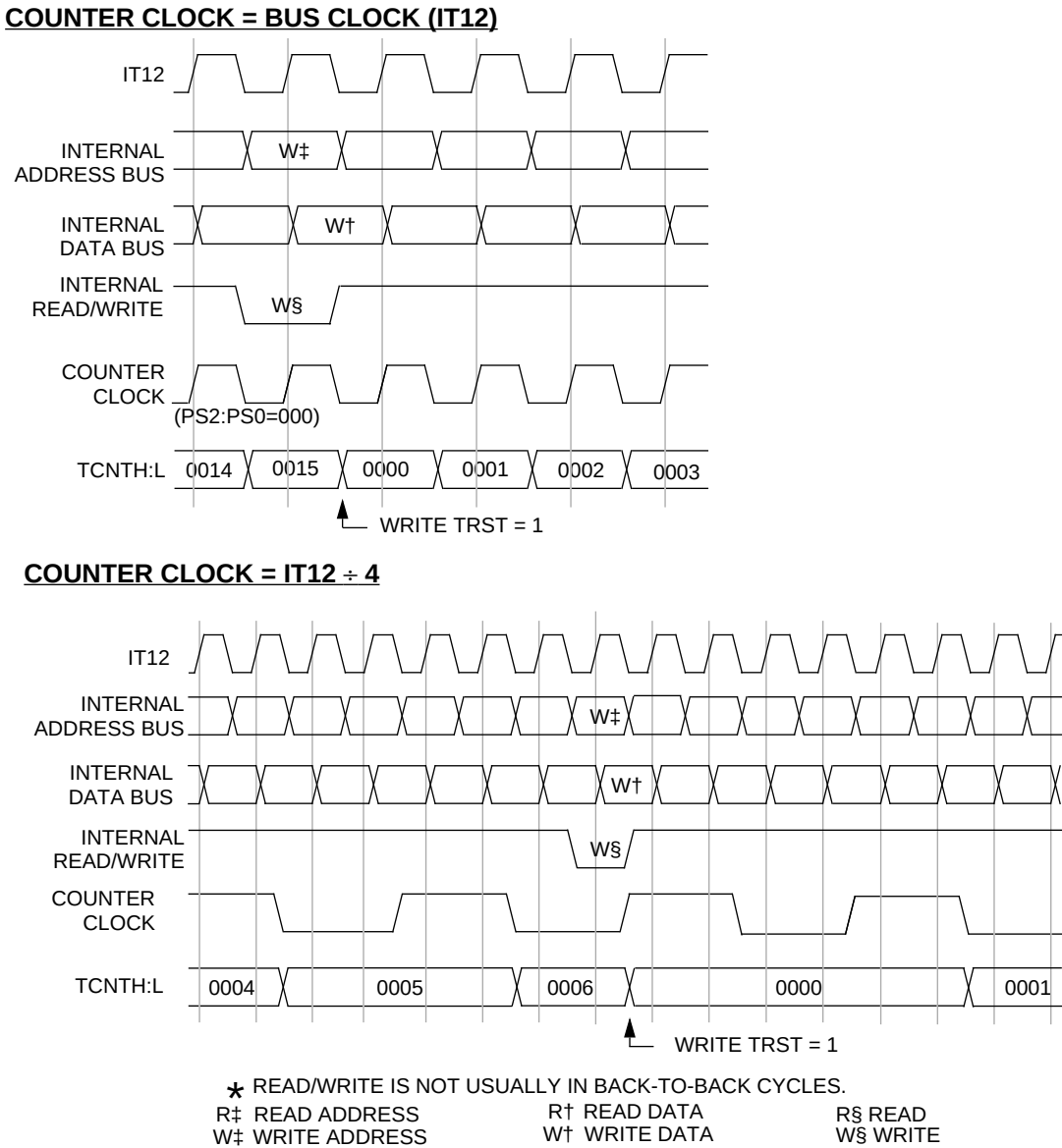
Figure 18. TRST Timing
