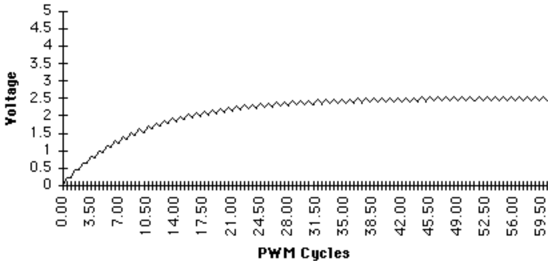
Figure 50. 10-kHz, 50% Duty Cycle RC Response
