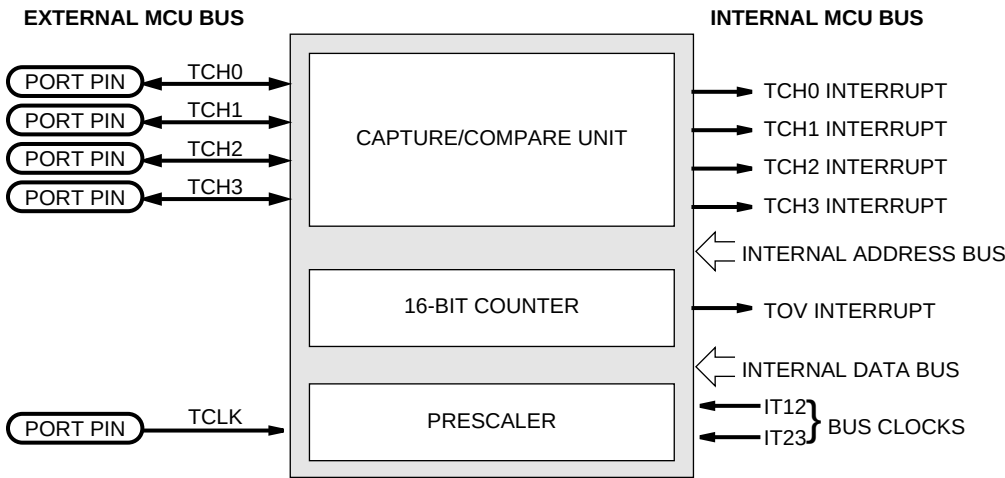
Figure 1. TIM Submodules
