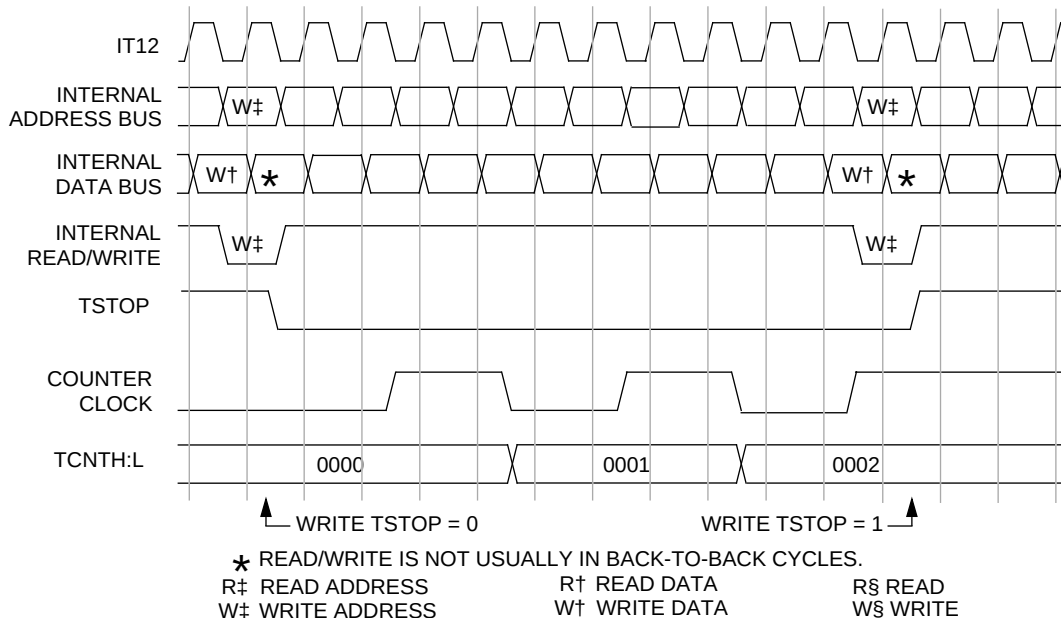
Figure 17. TSTOP Timing
