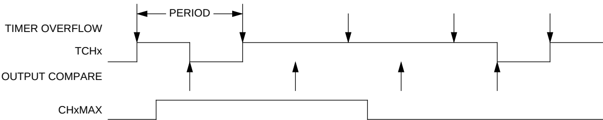
Figure 61. CHxMAX Latency
