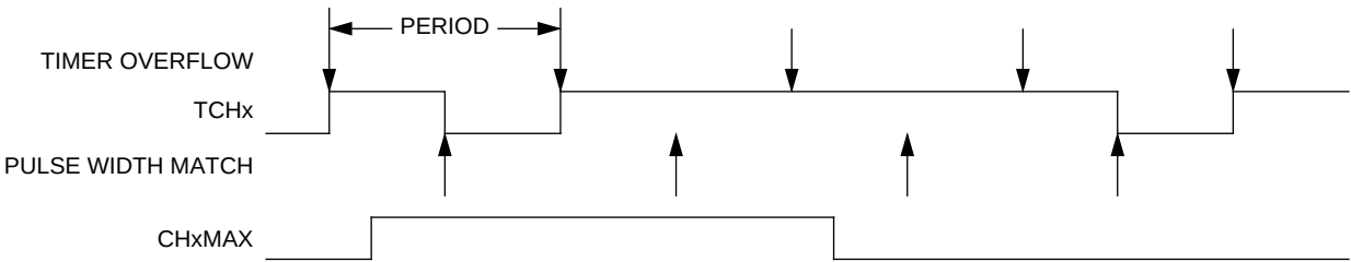
Figure 33. CHxMAX Latency
