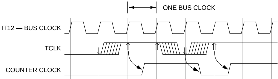
Figure 11. TCLK Timing
