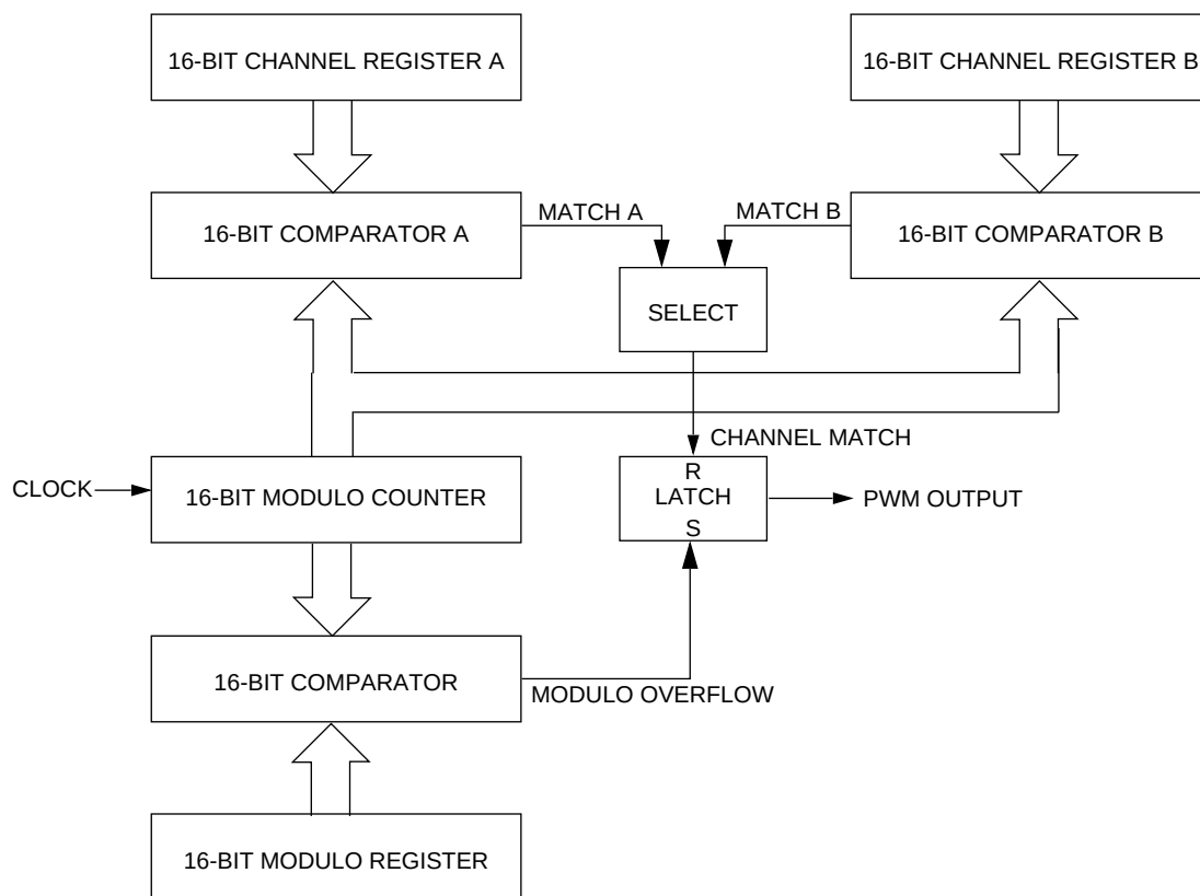
Figure 8. Buffered PWM Simplified Block Diagram
