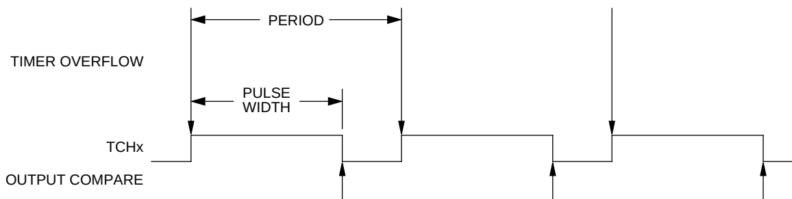
Figure 30. PWM Period and Pulse Width
