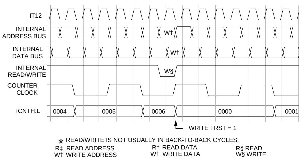
Figure 14. TRST Timing
