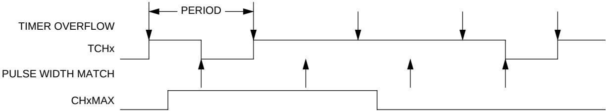
Figure 38. CHxMAX Latency
